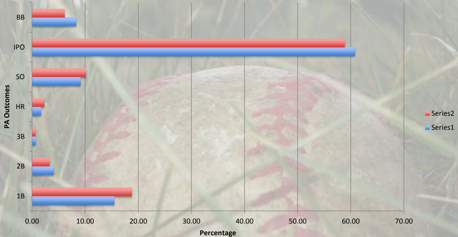
Side-by-Side Percentage
